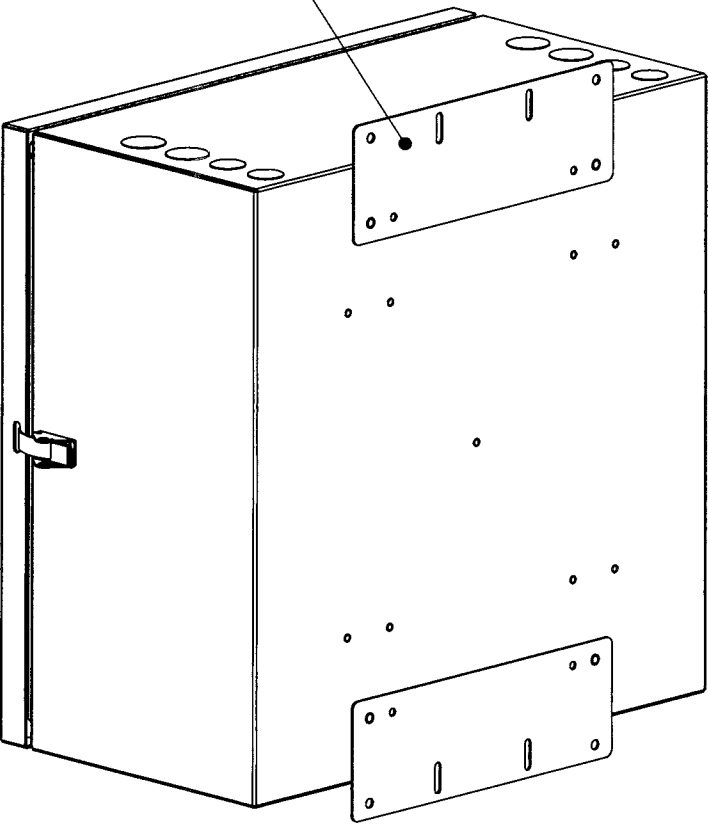
WALL MOUNT BRACKET TOP AND BOTTOM
