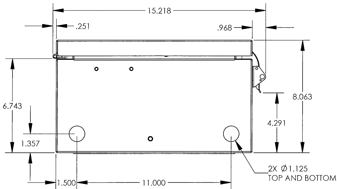
WALL MOUNT BRACKET TOP AND BOTTOM
